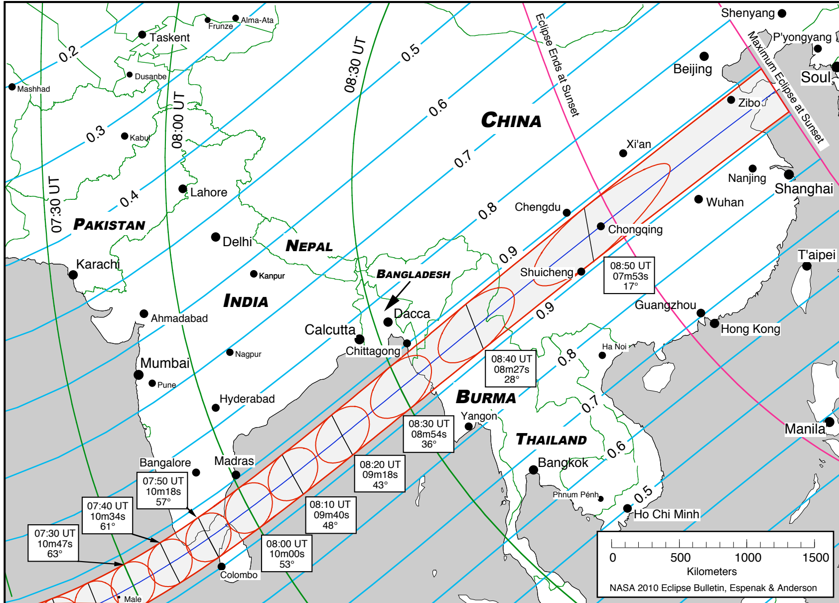
FIGURE 2.6: PATH OF THE ECLIPSE THROUGH ASIA
