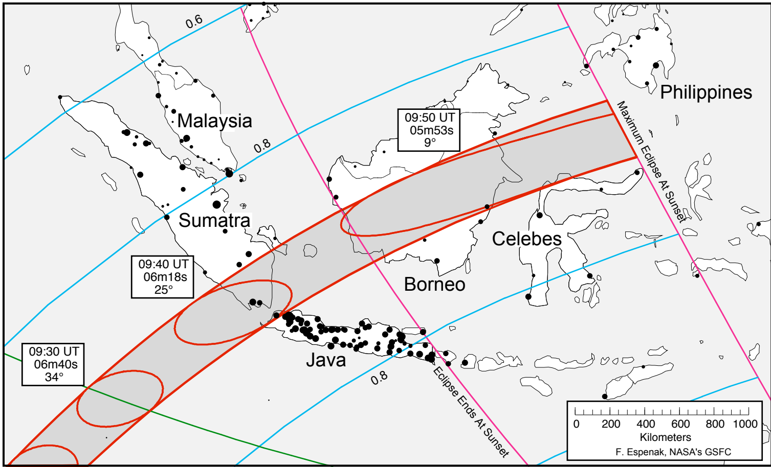
Figure 2: Path of Annular Solar Eclipse of 2009 Jan 26 Through Indonesia
