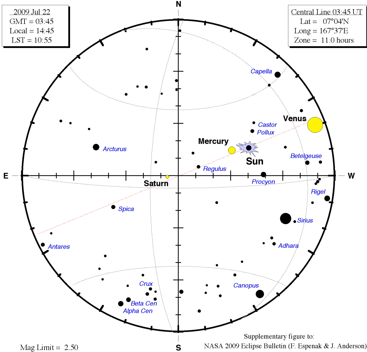
FIGURE 25D - SKY DURING TOTALITY AS SEEN FROM CENTRAL LINE AT 03:45 UT (FOR MARSHALL ISLANDS)
